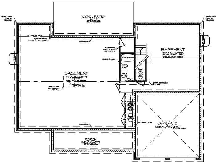
FOUNDATION PLAN SCALE: 1/4\"/>
