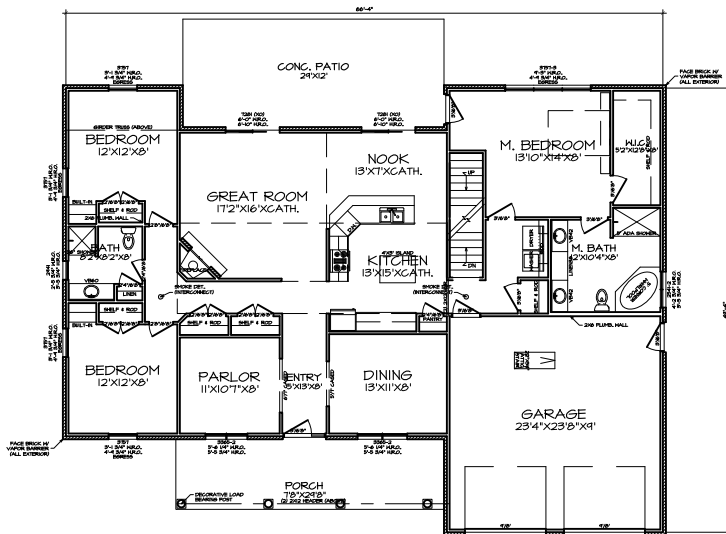
FIRST FLOOR PLAN A-2
