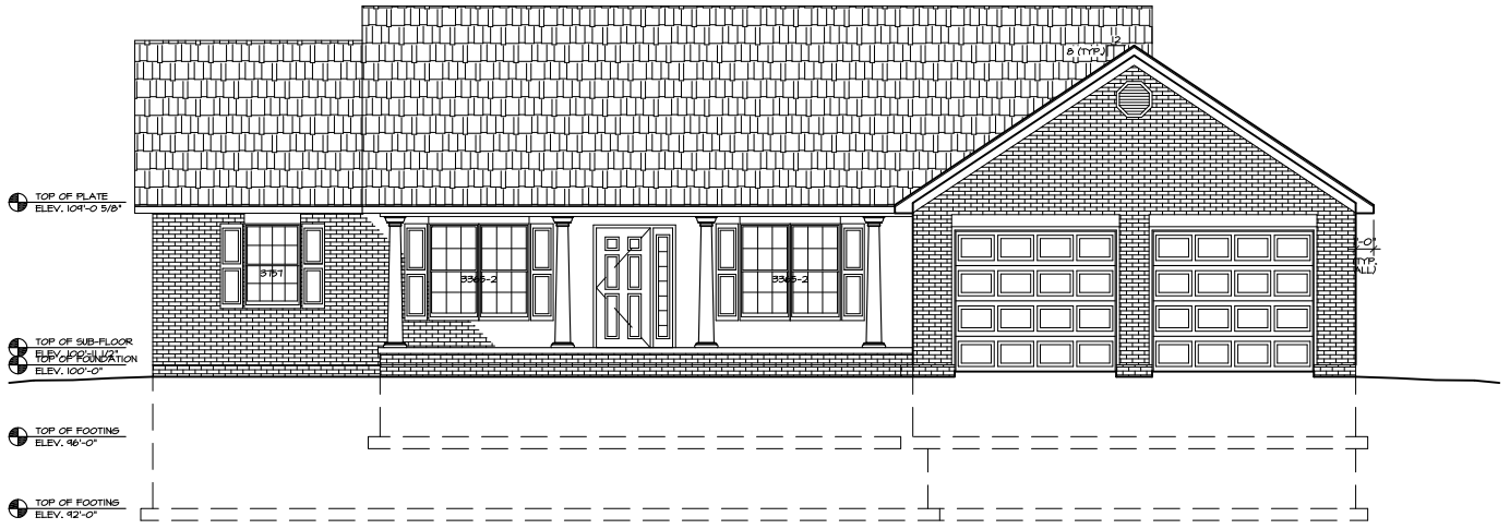
FRONT ELEVATION A-1
